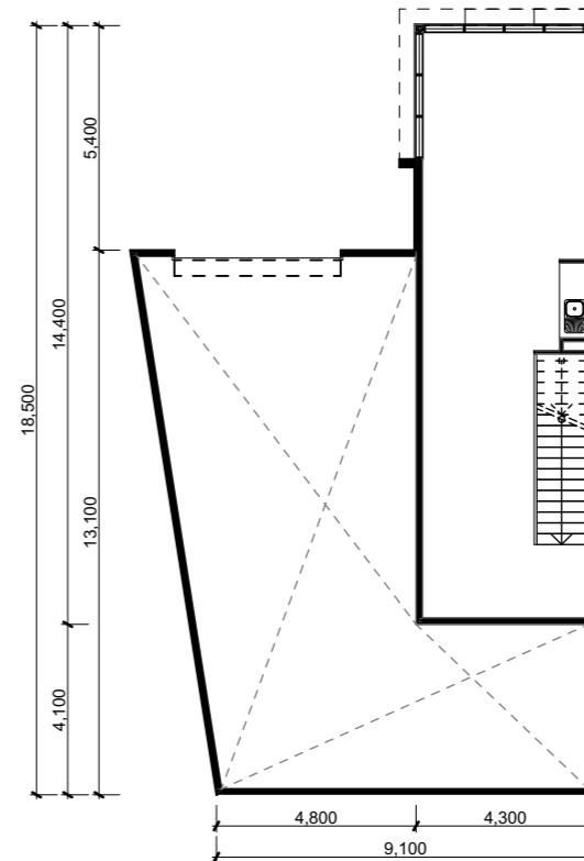
unit 215 first floor plan
